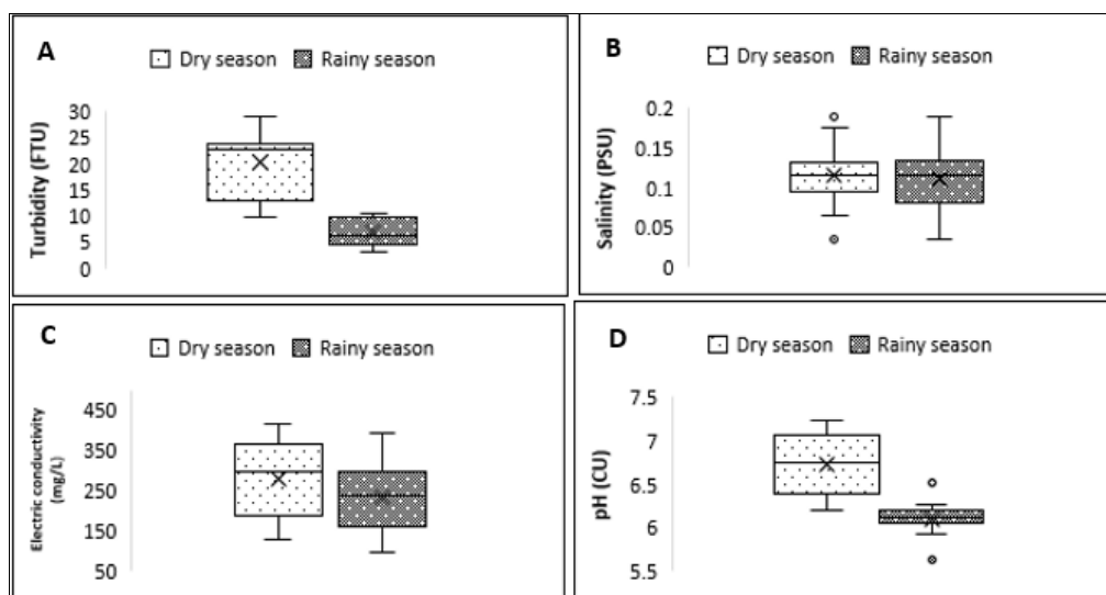
Fig 3: Boxplots showing the spatial and temporal distribution of turbidity (A), salinity (B), electric conductivity (C) and pH (D) in the wells studied in Tiko.
