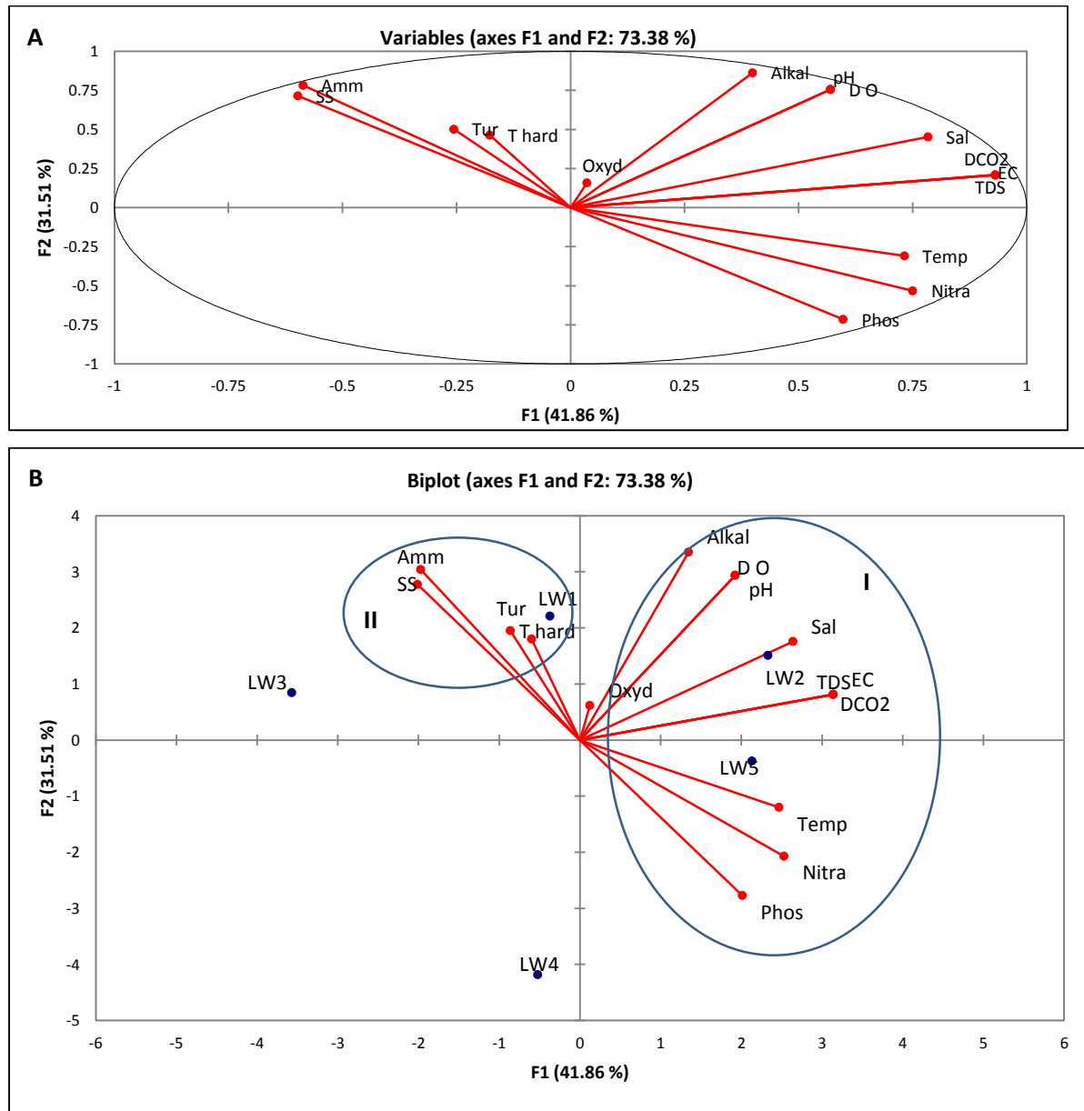
Figure 47: PCA of physicochemical parameters of the different sampling points during the study period in Limbe. (A) Circle of correlation between variables and factorial axes F1 and F2, (B) Biplot showing the distribution of samples in F1 and F2 factorial plan.
