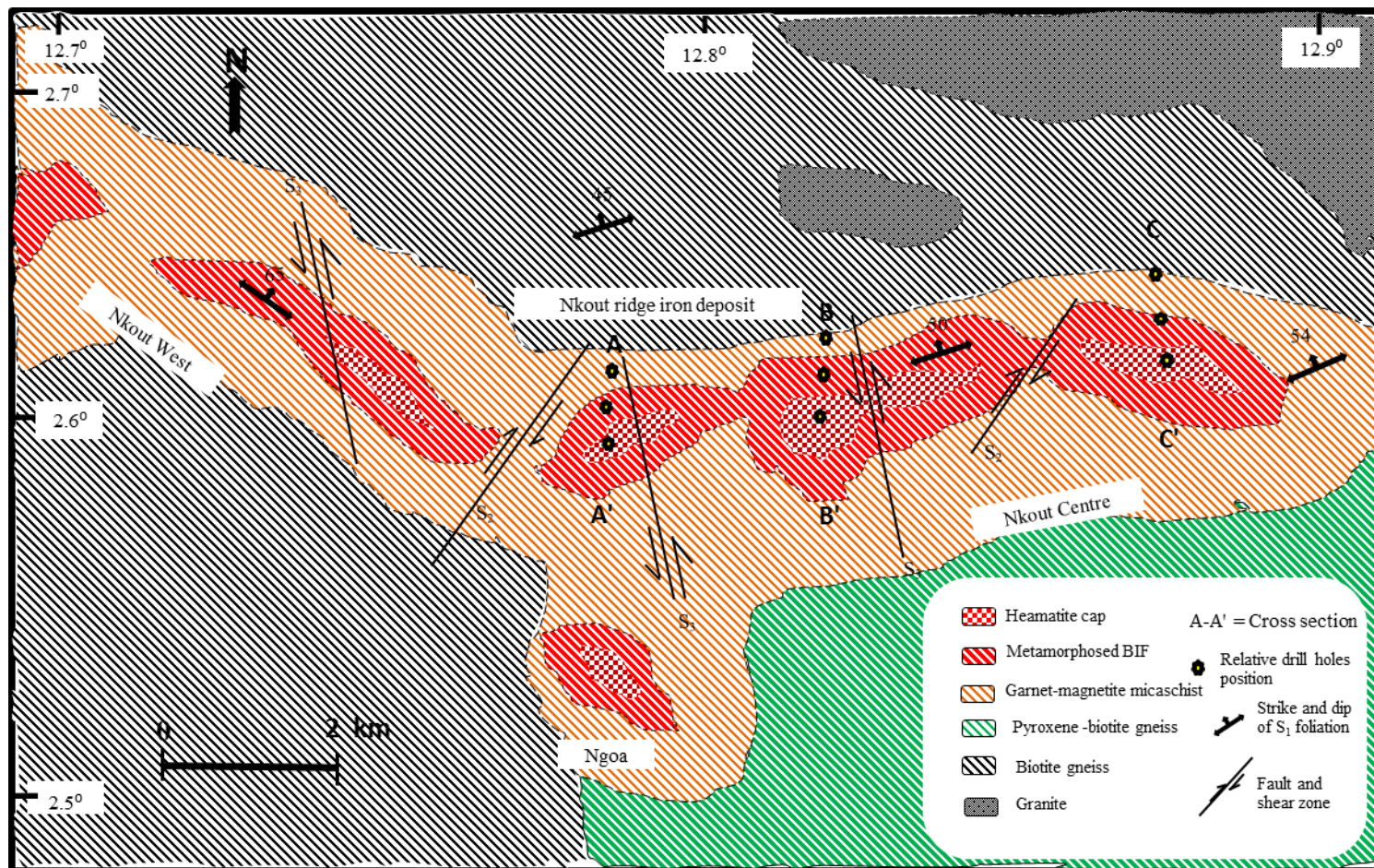
Figure 13: Local geological map of Nkout study area
