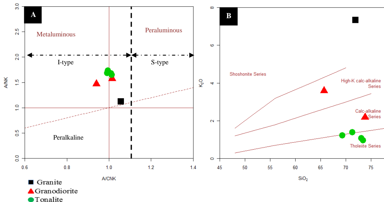
Figure 31: Geochemical characterization of Nkout plutonic rock (granite, granodiorite and tonalite): (a) \text{Al}_2\text{O}_3/(\text{CaO}+\text{Na}_2\text{O}+\text{K}_2\text{O}) versus \text{Al}_2\text{O}_3/(\text{Na}_2\text{O}+\text{K}_2\text{O}) moles% diagram showing metaluminous composition and (b) \text{K}_2\text{O} versus \text{SiO}_2 showing low-high \text{K}_2\text{O} (Peccerillo and Taylor 1976)
