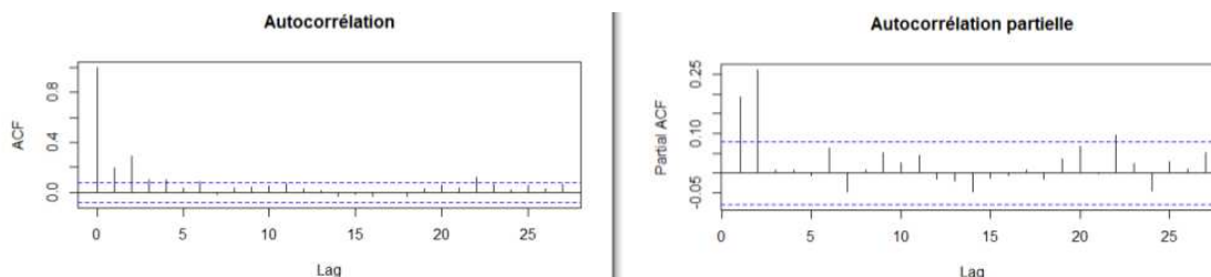
Figure 1: ACF and PACF for series \log(\text{iqa}) .
