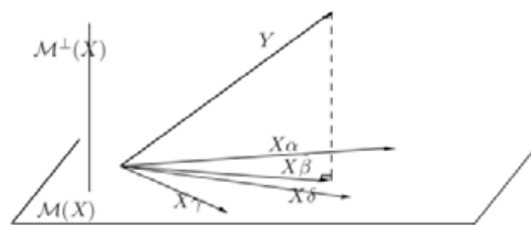
Figure 2: Representation \hat{X}\beta in variable space.
