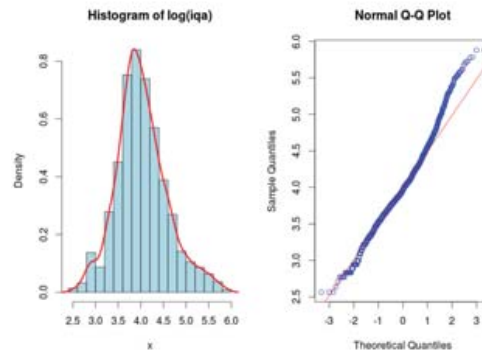
Figure 3: Residuals histogram and Q - Q plot of \log(iqa)
