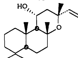
11β-hydroxymanoyloxyde 79
