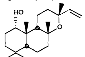
1α-hydroxymanoyloxyde 80
