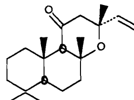
11-oxomanoyloxyde 75
