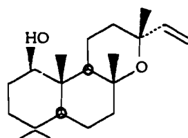
1β-hydroxymanoyloxyde 81
