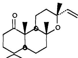
1-oxo-manoyloxyde 77
