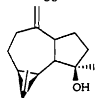
1α-hydroxymanoyloxyde 80
