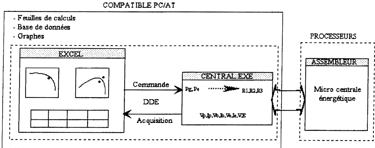
Figure 3.15: Principe de la supervision
