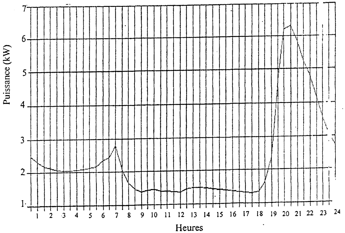
Figure 5. 12: Courbe de charge Ndiébel
