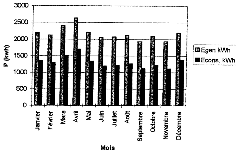
Figure 5. 5: Variation annuelle Production/Consommation
