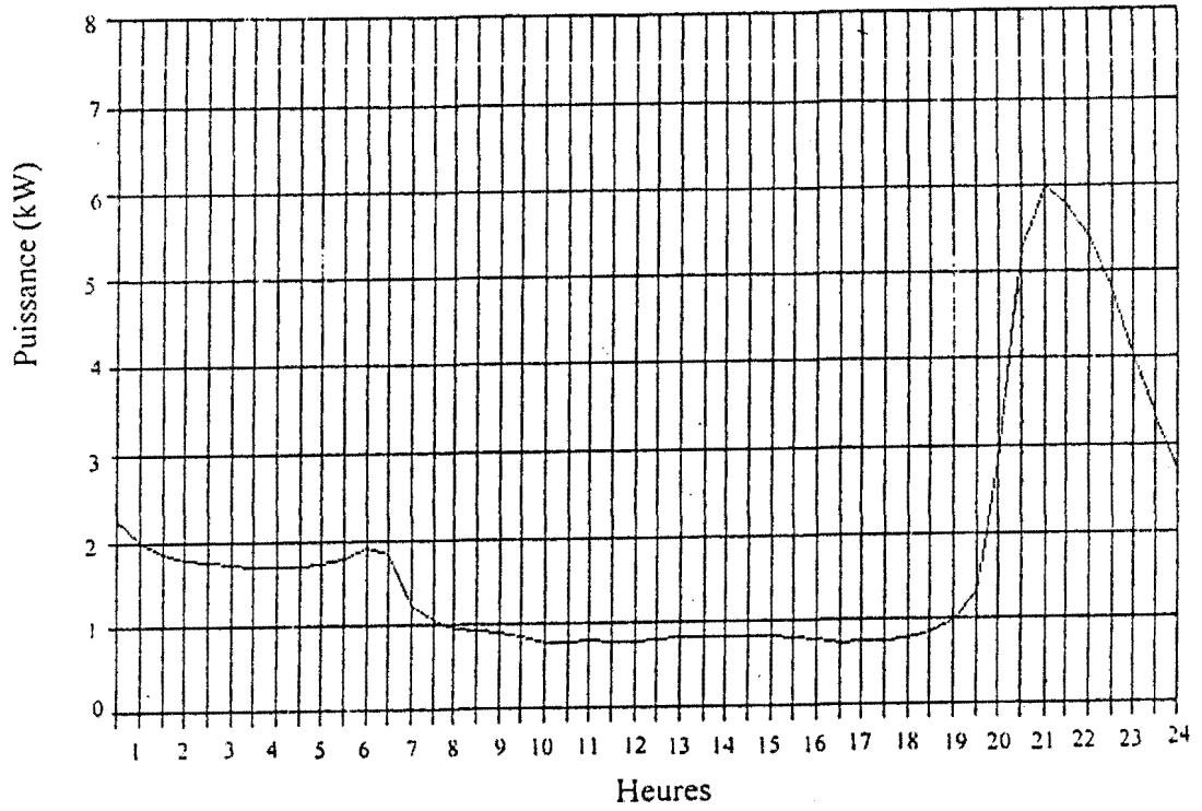
Figure 5. 12: Courbe de charge Ndiébel
